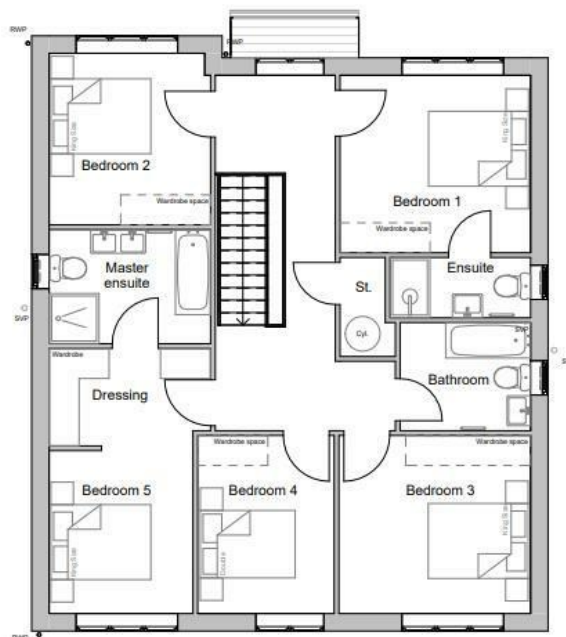
First Floor - GA Plan
