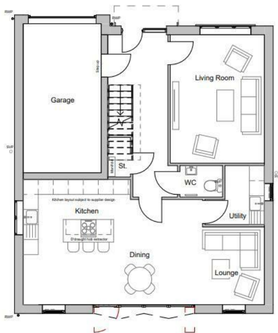
Ground Floor - GA Plan
